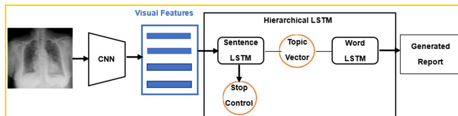
Fig. 5 Hierarchical RNN-based framework for medical report generation
